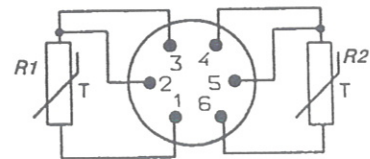
Pin assignment 2xPt100
