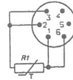
Pin assignment 1xPt100
